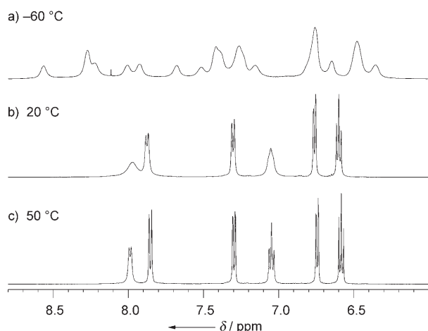
Figure 3. Aromatic region of the 1 H NMR spectra of [2C-Ga 4 L 6 ] 11- showing the signals for the 72 aromatic protons of the host at a) -60 °C in MeOD, b) room temperature in D 2 O, and c) 50 °C in D 2 O.
